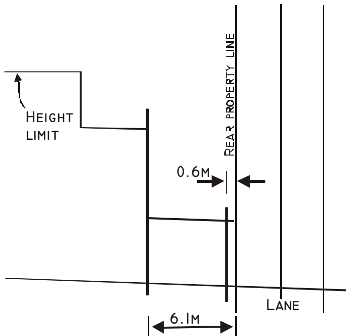
Figure 4 – Rear Yard and Setback
