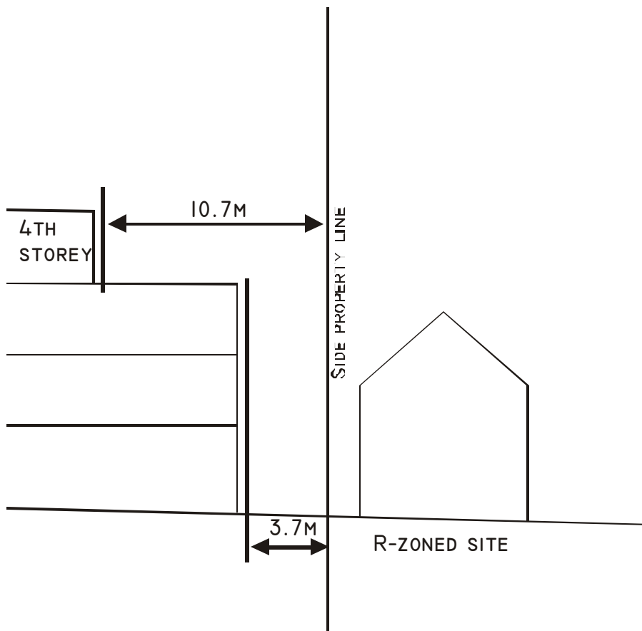
Figure 3 – Side Yard and Setback Adjacent to R-zoned Site
