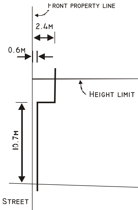
Figure 2 – Front Yard and Setback
